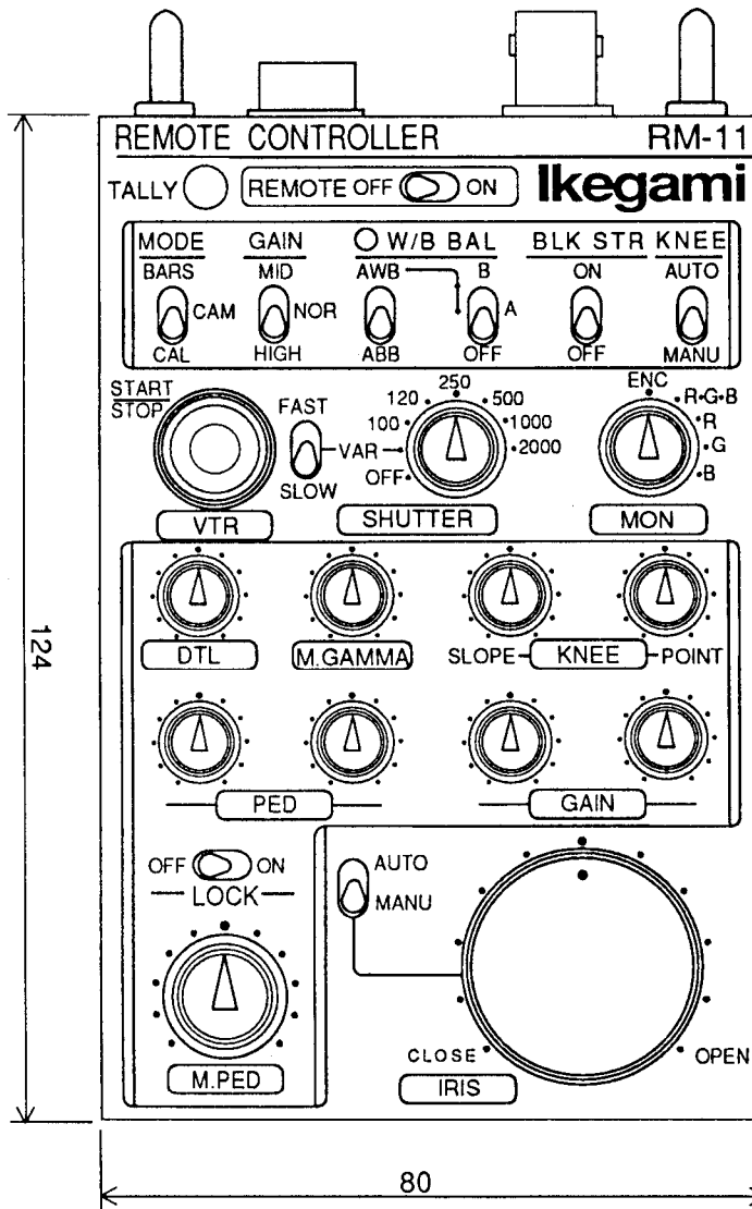
RM-11 (REMOTE CONTROLLER) External Appearance
