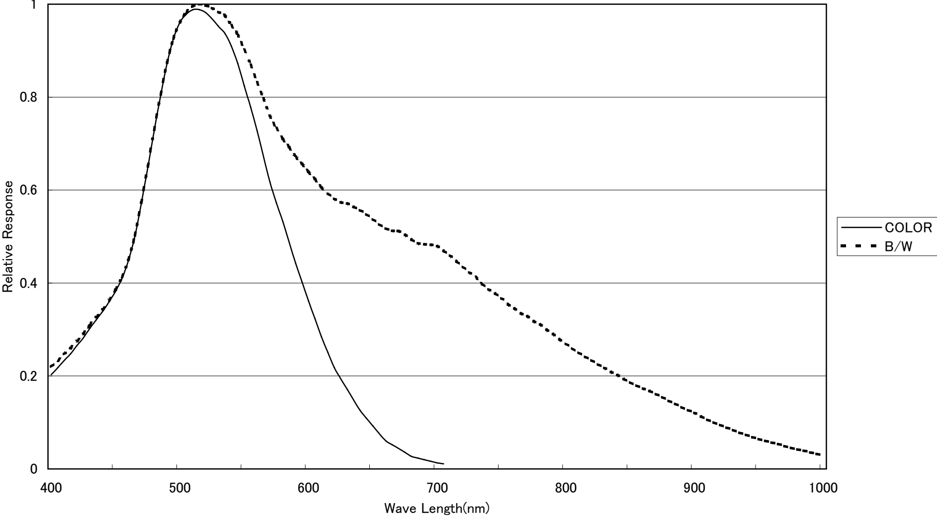
ICD-509/509P Spectral Response
