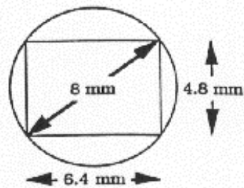
1/2" Camera Image Size
