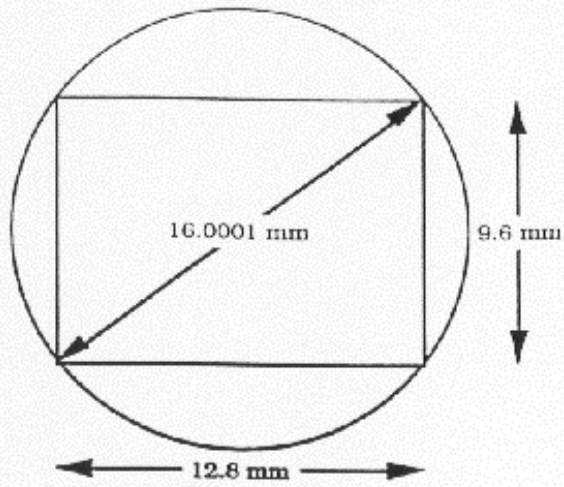
1" Camera Image Size
