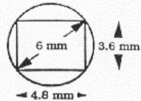
1/3" Camera Image Size
