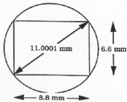
2/3" Camera Image Size
