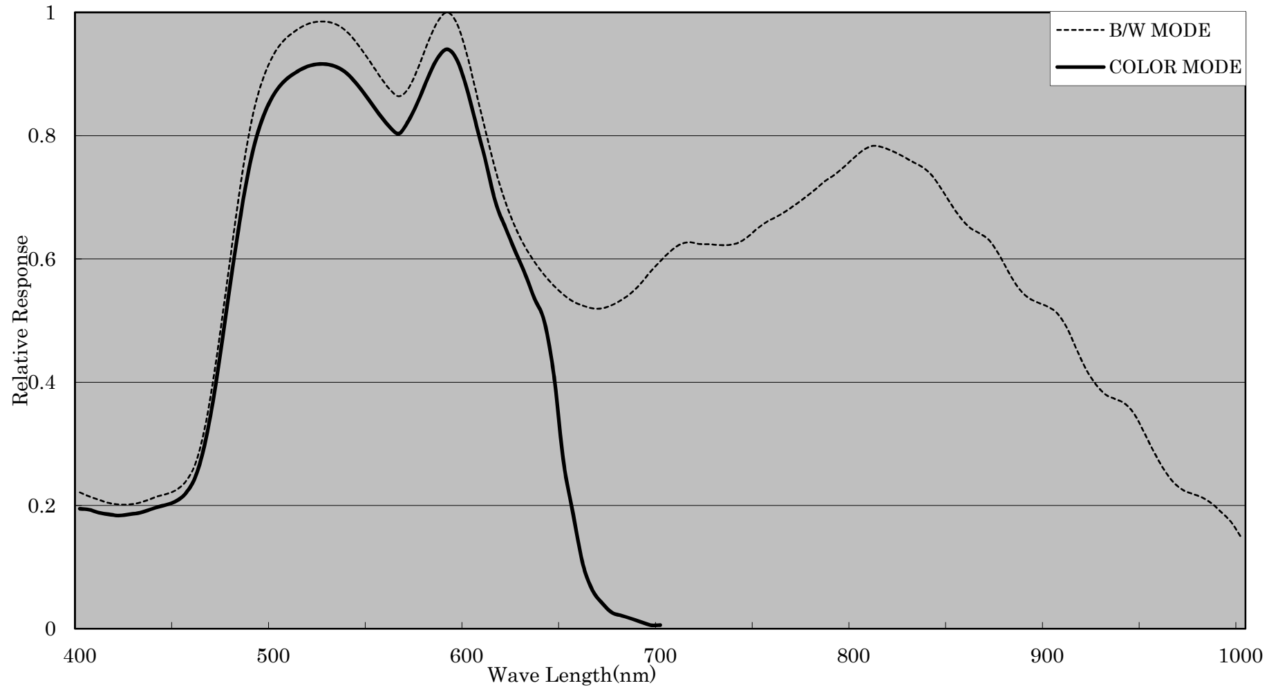
ISD-A15S Spectral Response
