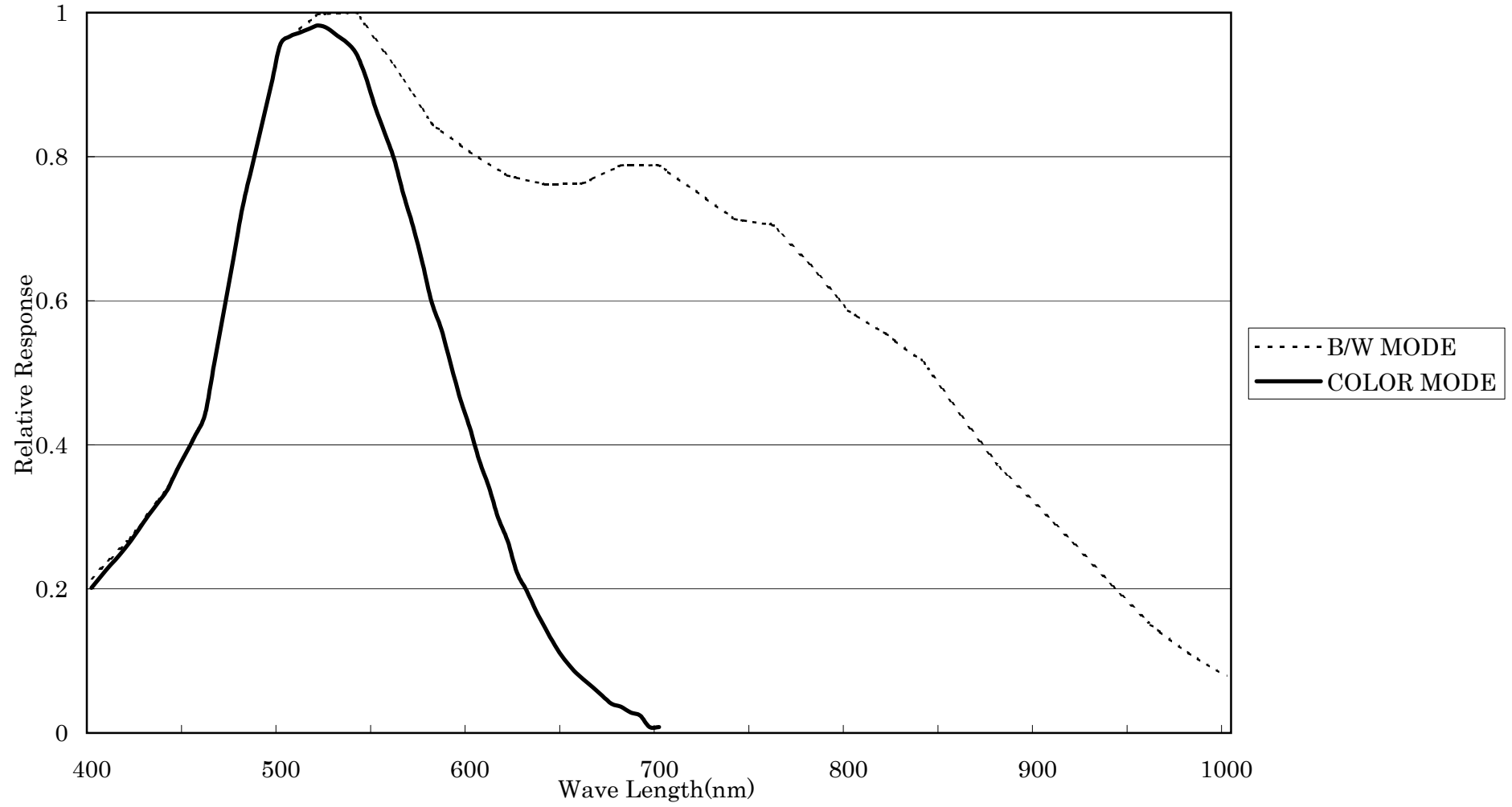
ICD-879/879P Spectral Response
