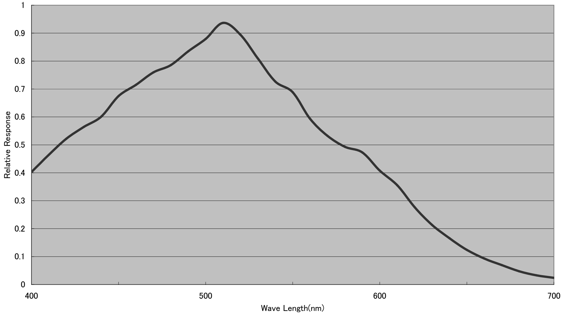
ISD-A14, ISD-A15, ISD-A33 Spectral Response
