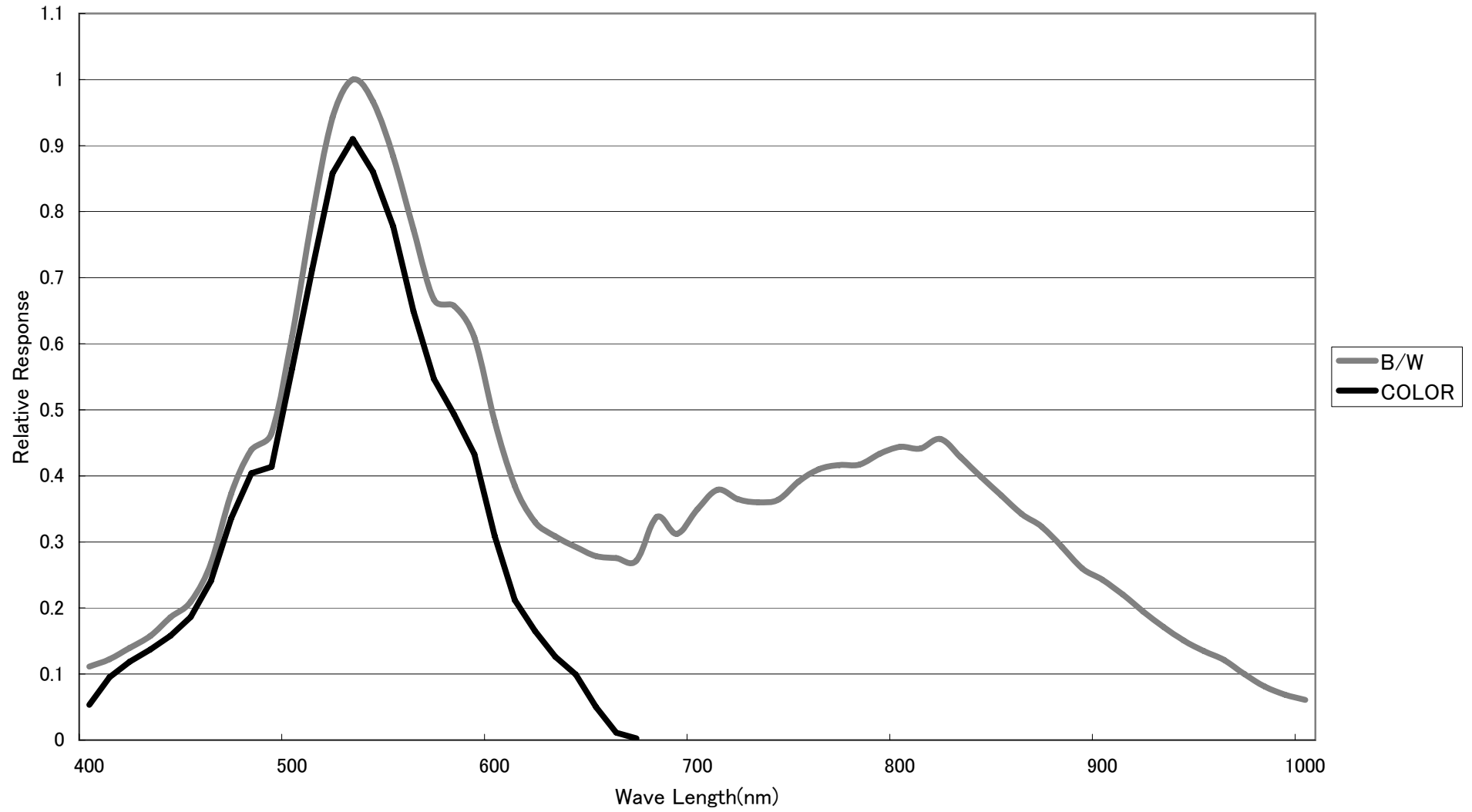
IPD-BX110 Spectral Response
