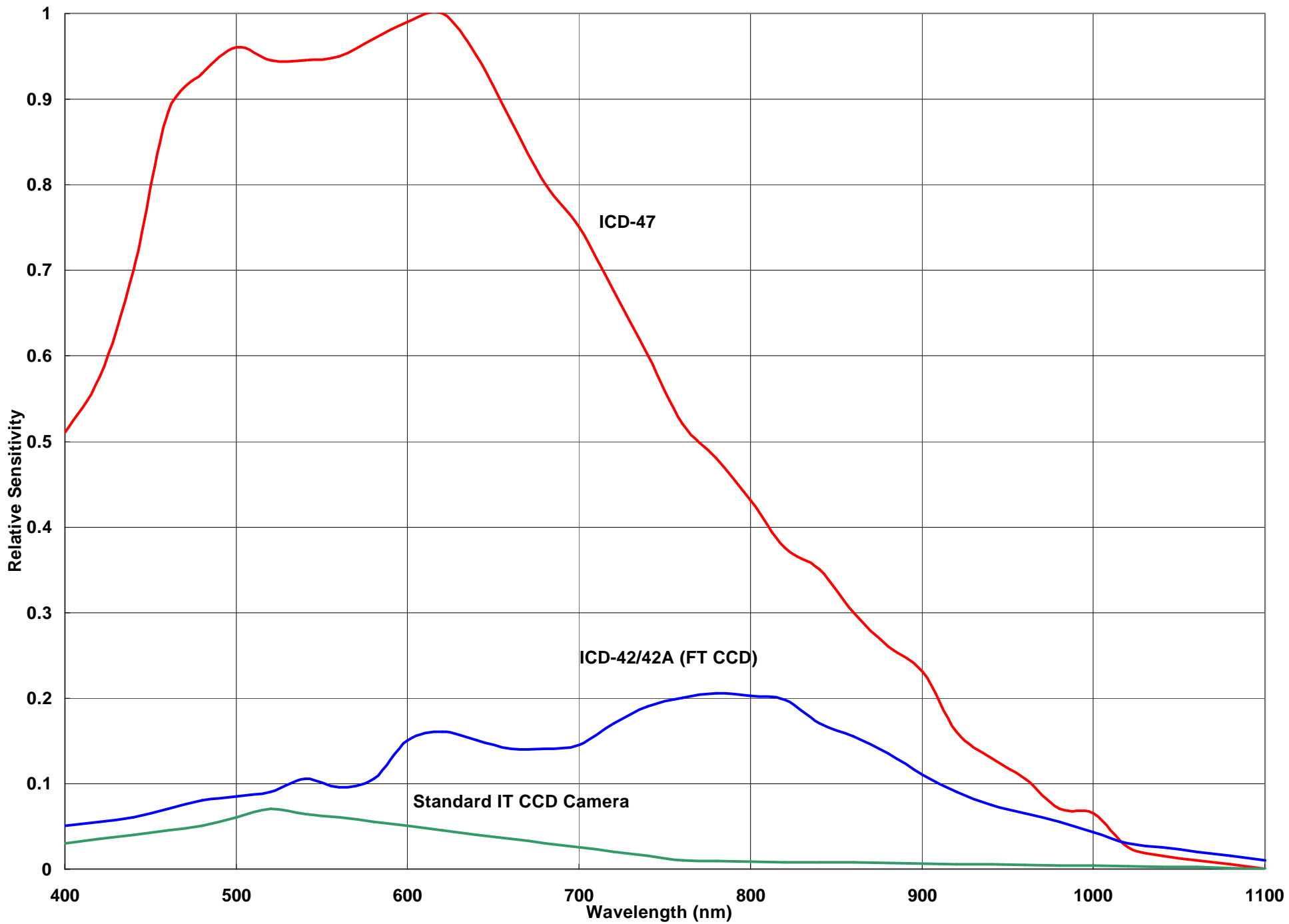
ICD-47 vs ICD-42,42A. Standard IT CCD Camera Relative Spectral Response and Sensitivity Comparison (AGC Maximum.)
