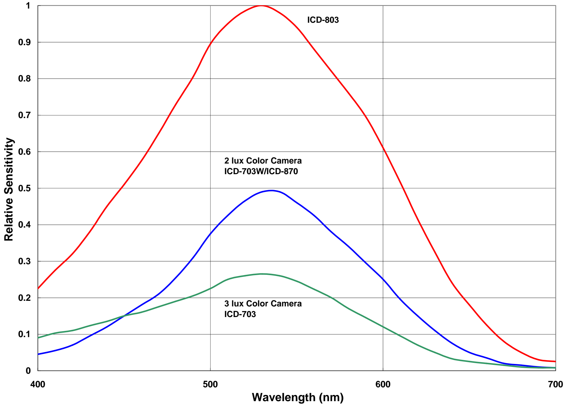
Color CCD Camera Relative Spectral Response and Sensitivity Comparison (AGC Maximum)
