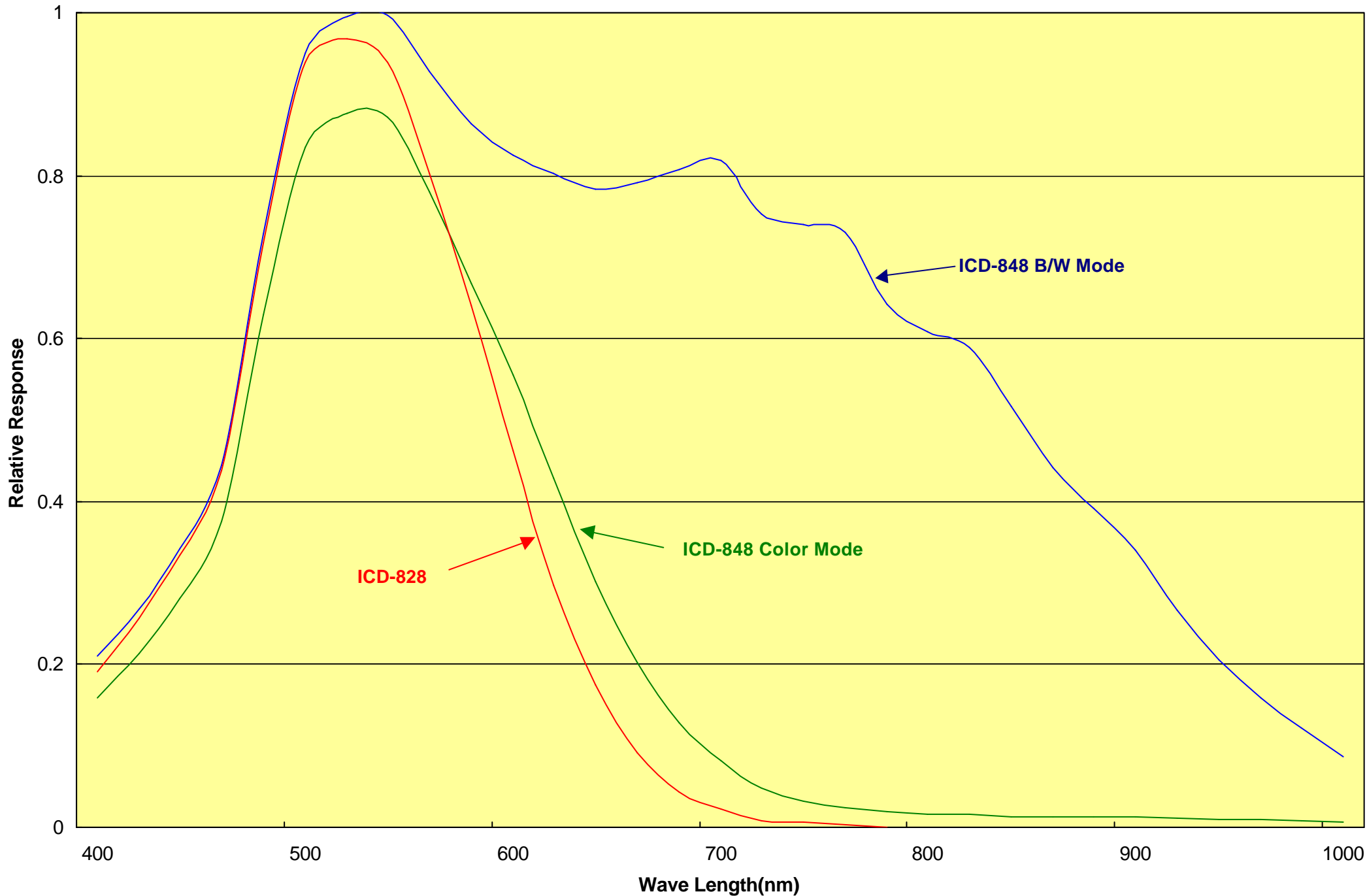
ICD-828/828P/848/848P Spectral Response
