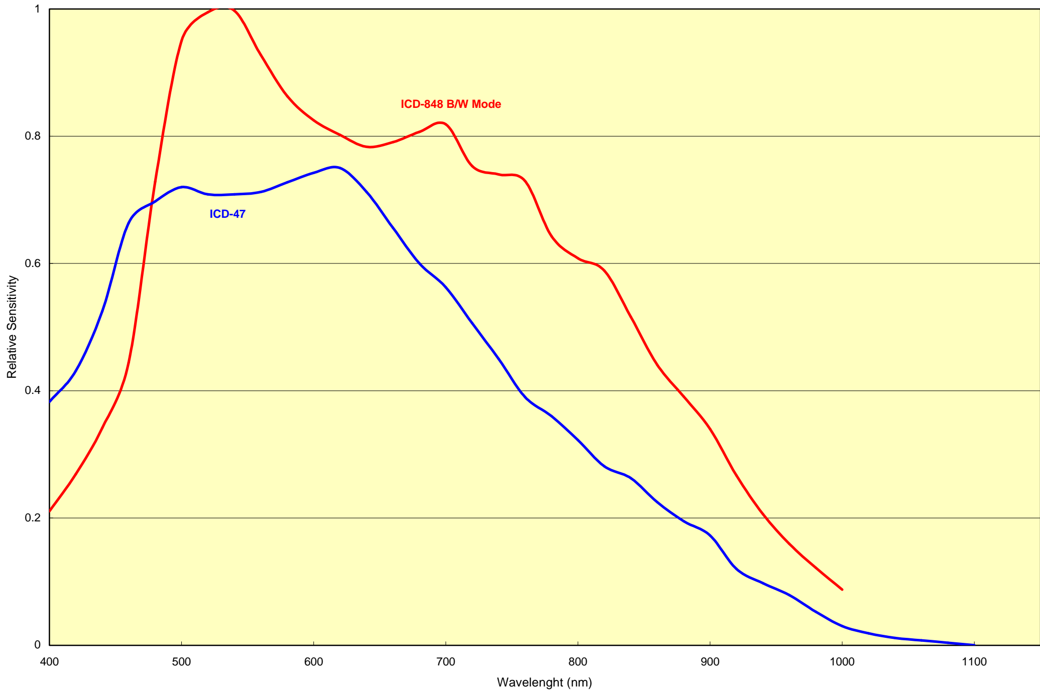
ICD-848 (B/W Mode) vs ICD-47 Spectral Response Data
